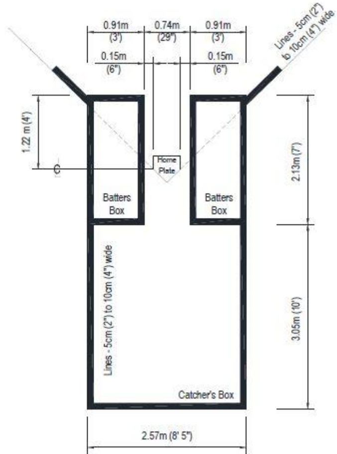
BATTER AND CATCHERS BOX DETAIL
